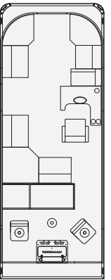
240 FISH N' CRUISE 243 FISH N' CRUISE
